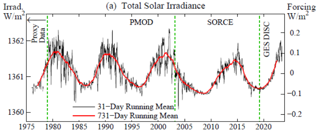
Fig. 6. Solar irradiance and climate forcing, the latter being 0.175 \times irradiance change, where 0.175 = (1 - \text{Earth's albedo})/4 , where Earth's albedo = 0.3 . Data sources: Physikalisch Meteorologisches Observatorium, Davos , University of Colorado Solar Radiation and Climate Experiment , and Total Irradiance Monitor on the International Space Station (GES DISC).
